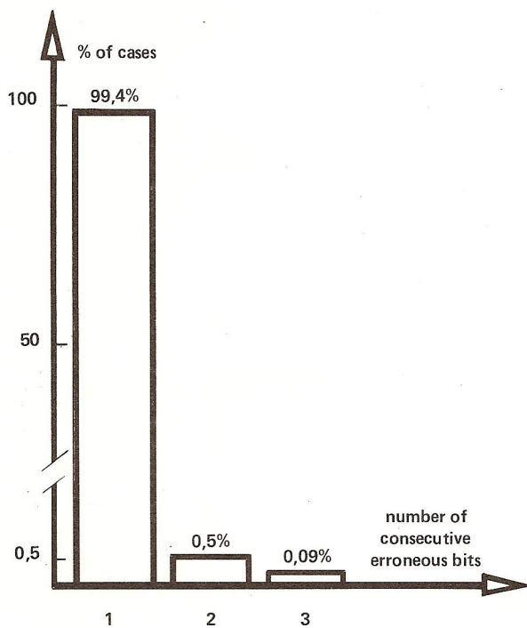
Length of observed errors
