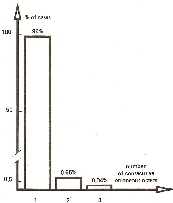
Length of consecutive erroneous octets
